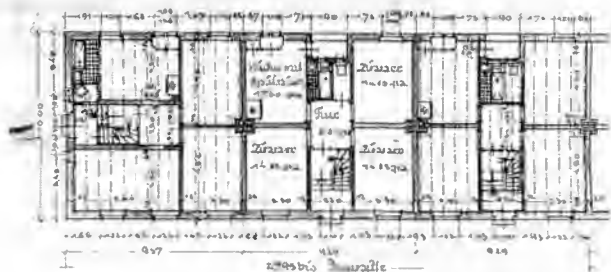
Erdgeschoss.
